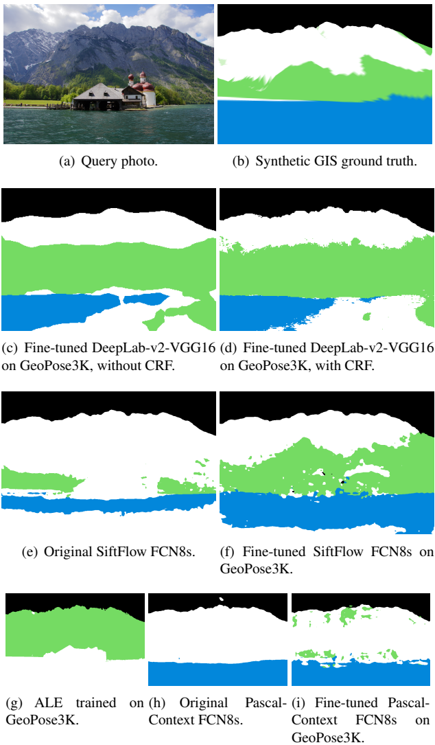
Figure 2. Illustration of mountain scene semantic segmentation using DeepLab-v2 based on VGG-16 model, before, and after fine-tuning on the GeoPose3K dataset.
