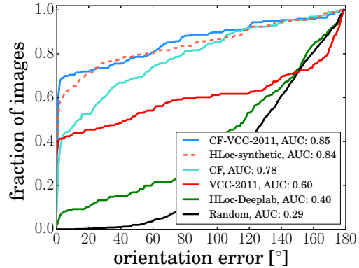
Figure 3. CH1 dataset: Comparison of the edge-based VCC-2011, our CF framework using semantic segments, and combination of both approaches. We use our CF framework to fuse semantic segments and edges together (CF-VCC-2011), which gives the best result.
