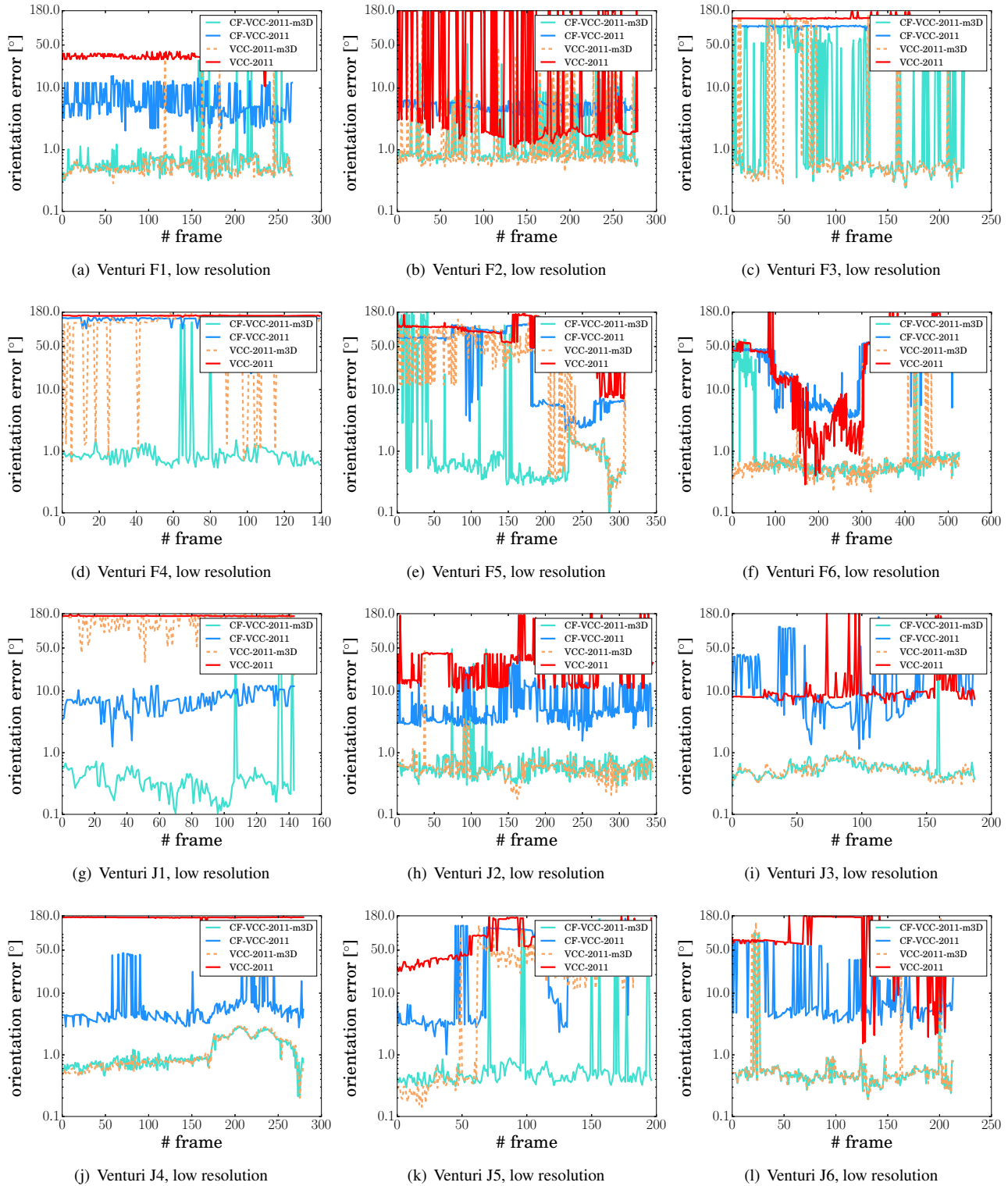
Figure 4. Per-frame orientation error on Venturi mountain dataset (low resolution).
