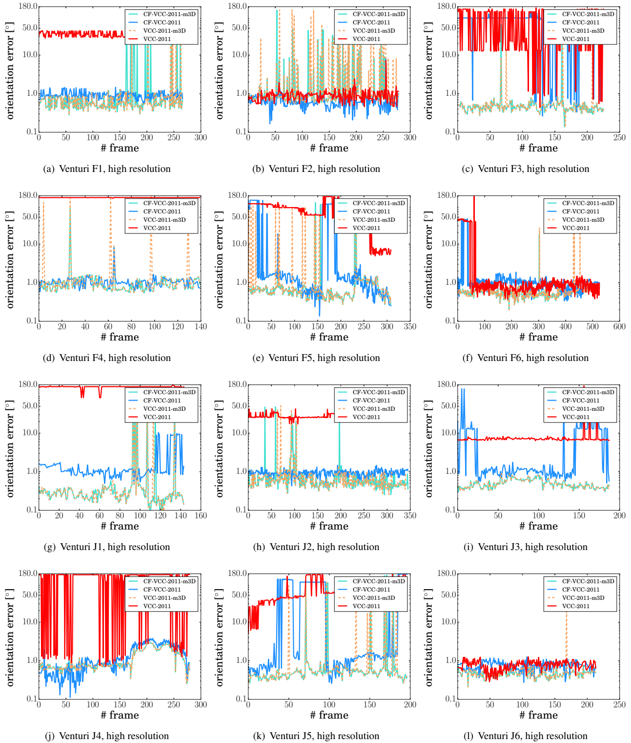
Figure 5. Per-frame orientation error on Venturi mountain dataset (high resolution).
